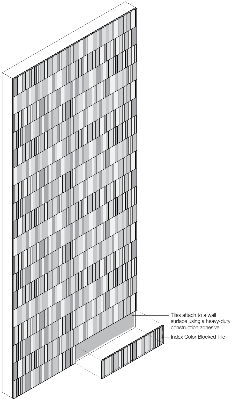
Exploded Axonometric Four Modules in Standard Pattern
